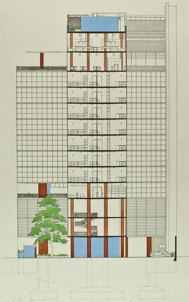
sectional elevation
