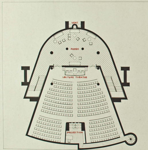
basement
