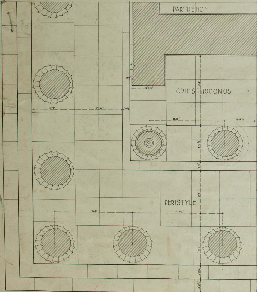
PLAN OF NORTH-WEST CORNER
