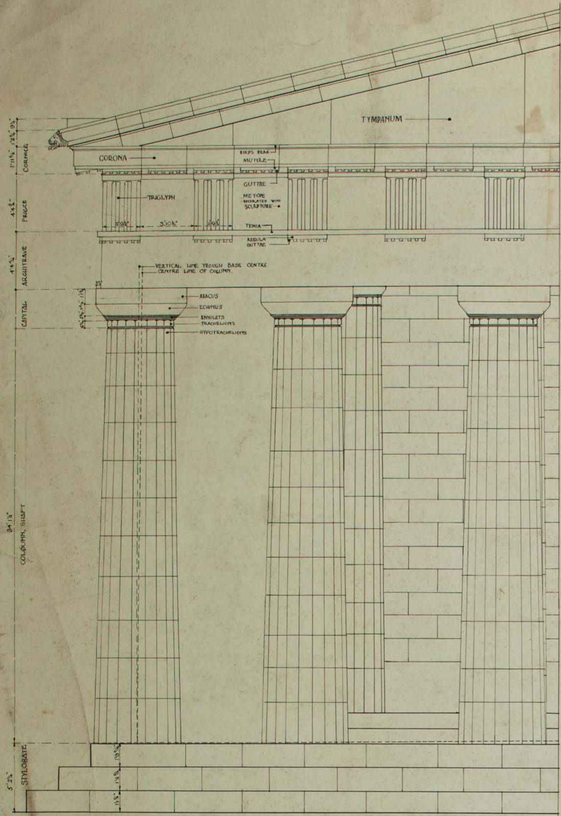
PART - WEST ELEVATION
