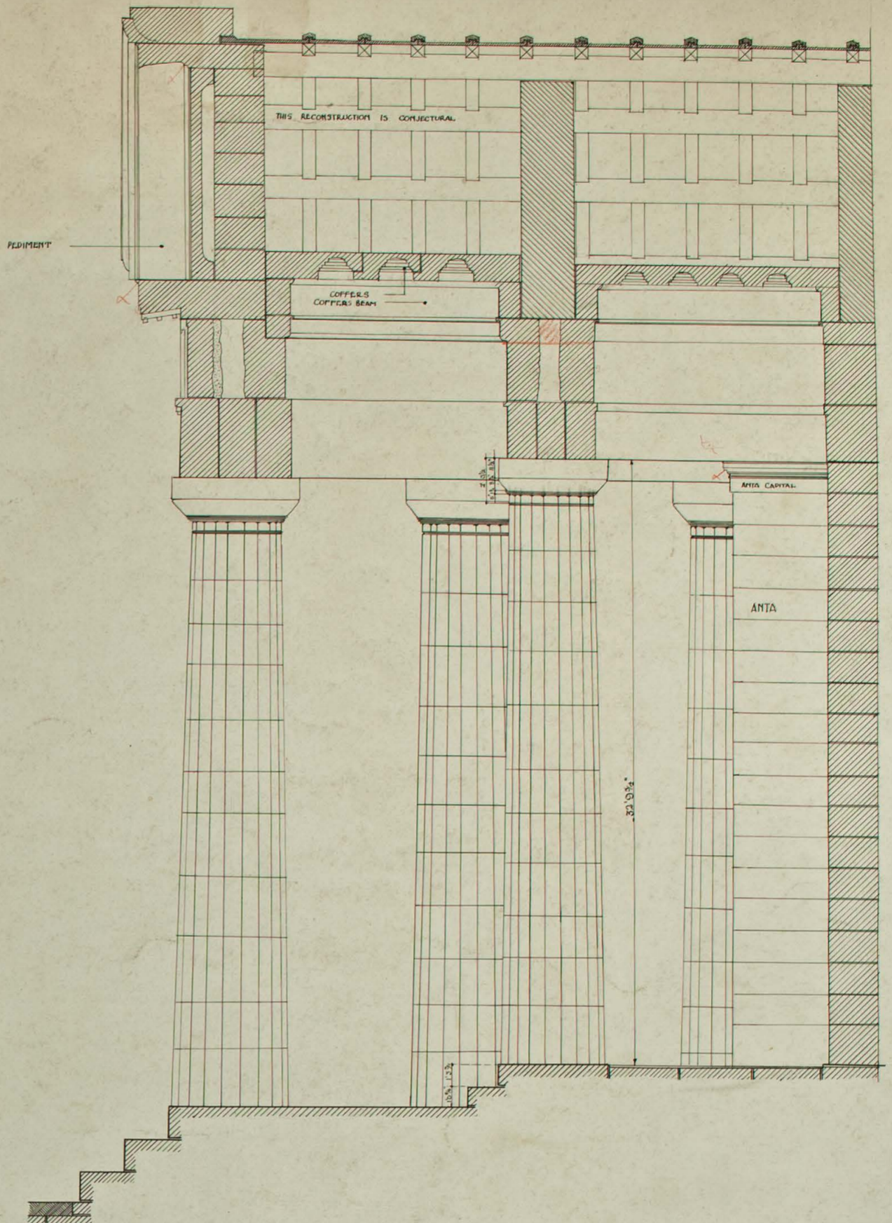
PART - LONGITUDINAL SECTION ON CENTRE LINE - RESTORED
